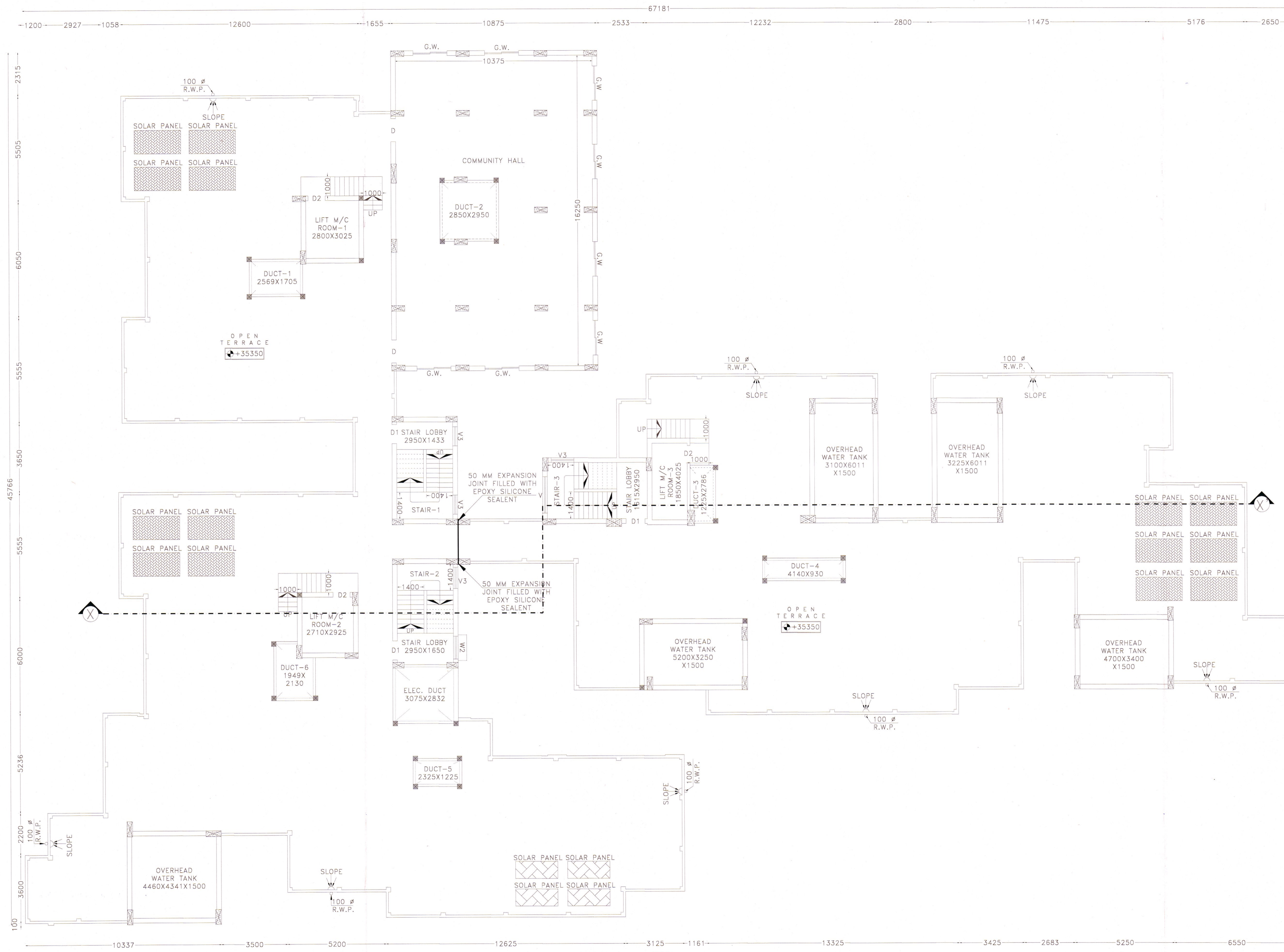
E ROOF FLOOR PLAN SCALE: 1:100
